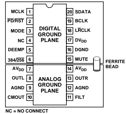
Figure 22. Recommended Ground Plane
